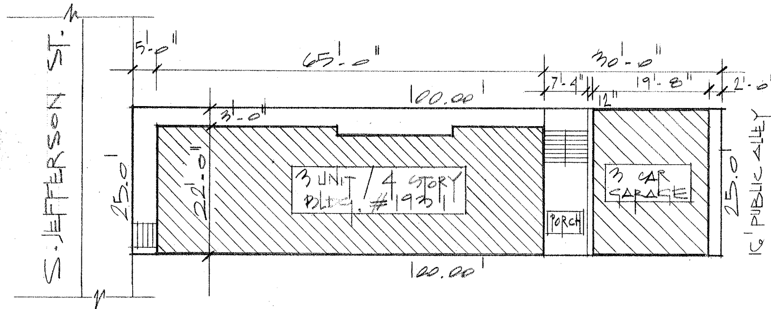
⊕ SITE PLAN 1/16" = 1'-0"
